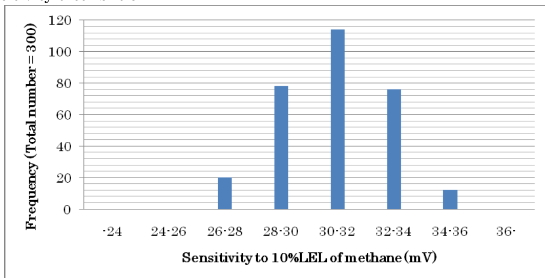
Fig. 9 : Sensitivity distribution
